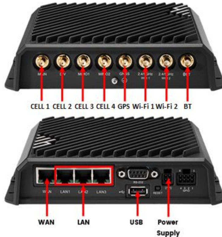
Figure 8: Cradlepoint R1900 Connections
