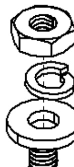
Figure 4: For R1900 router, fasten the router to the cover plate PTA0579 screws, PTA0140 washers, PTA0844 lock washers, and PTA0408 nuts.
