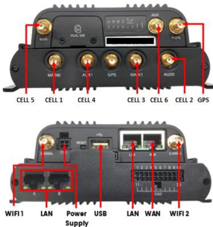
Figure 7: Cradlepoint IBR900 with COR Extensibility Dock Connections
