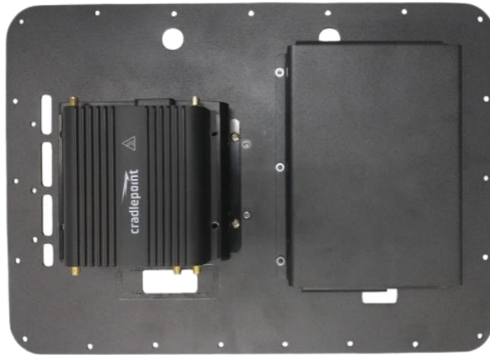
Figure 3: For IBR900 router, fasten the router to the cover plate using PTA0399-TL screws.
