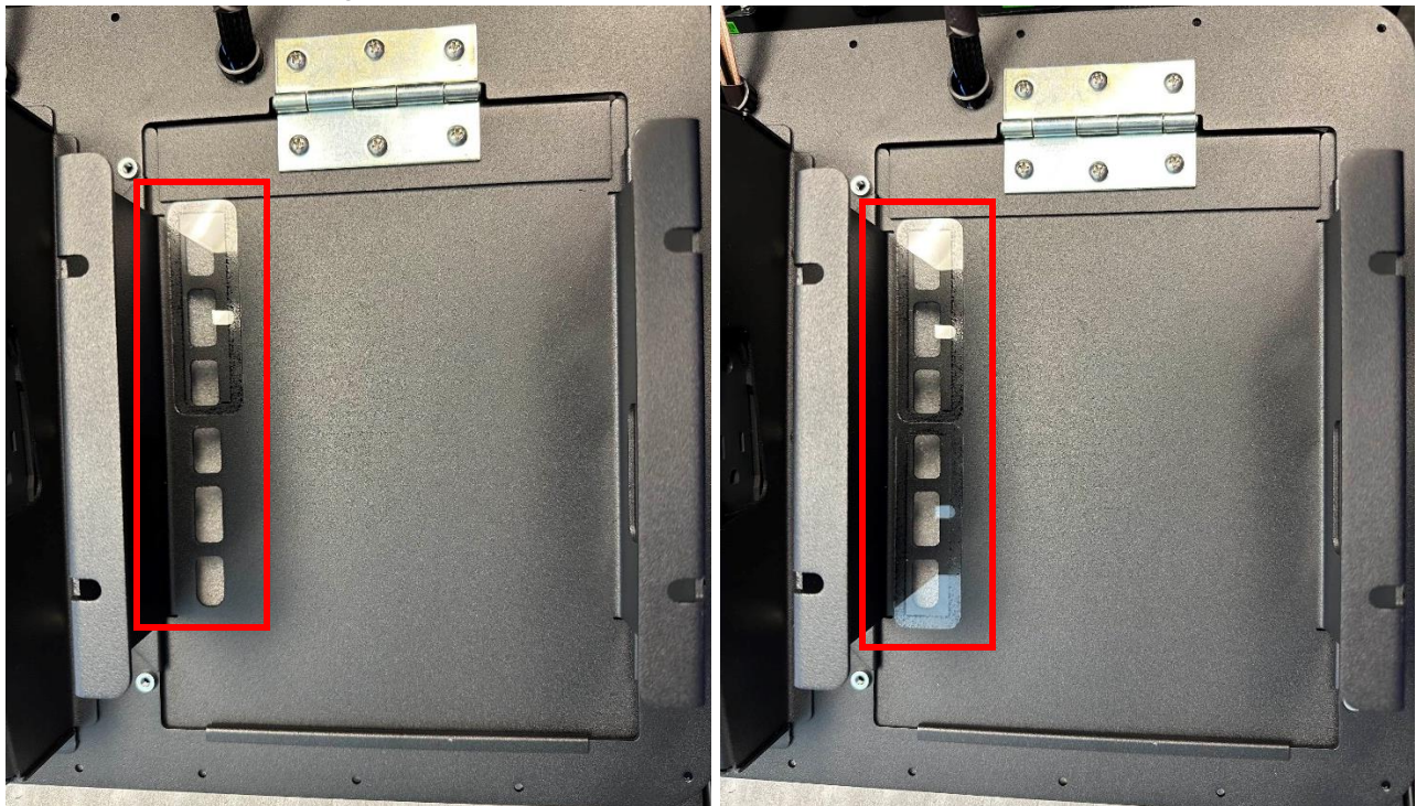
Figure 5: Install the Display Covers on the Cover Plate.
