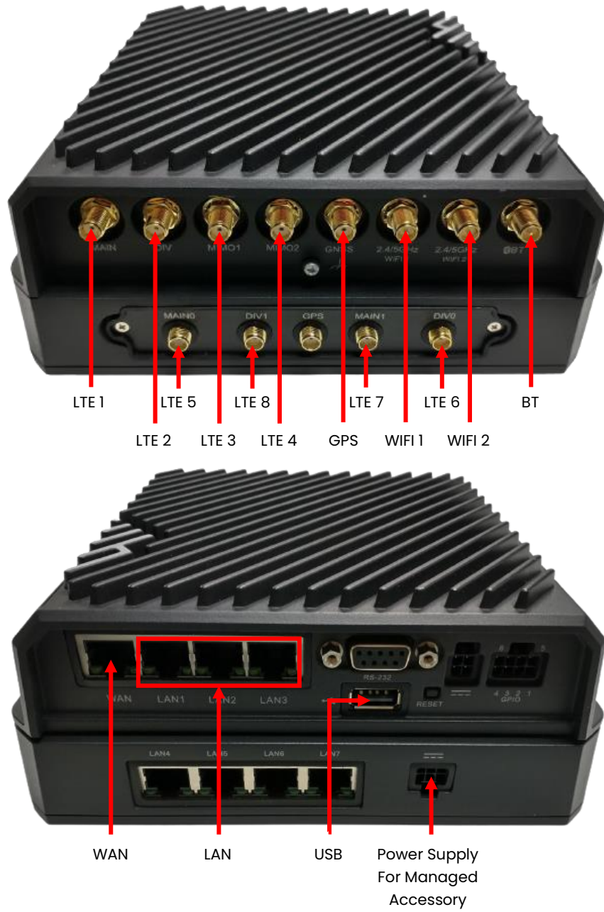
Figure 9: Cradlepoint R1900 Connections
