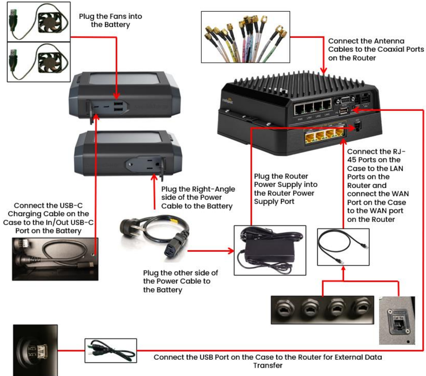
Figure 8: Connection Diagram for Bloodhound R19D
