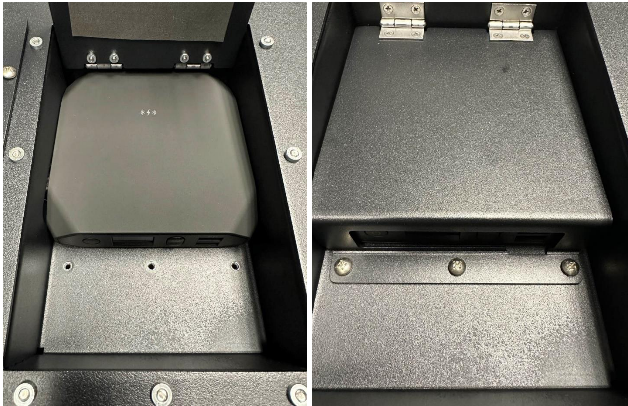
Figures 1-2: Insert the battery pack into the battery tray and secure the Battery Tray.
