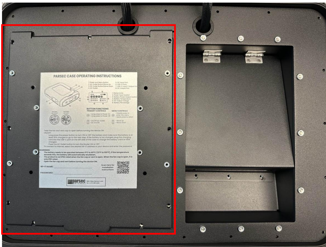
Figure 5: Remove the Router Plate from the Cover Plate
