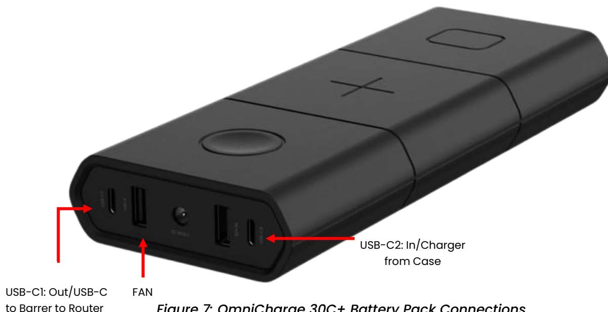
Figure 7: OmniCharge 30C+ Battery Pack Connections
